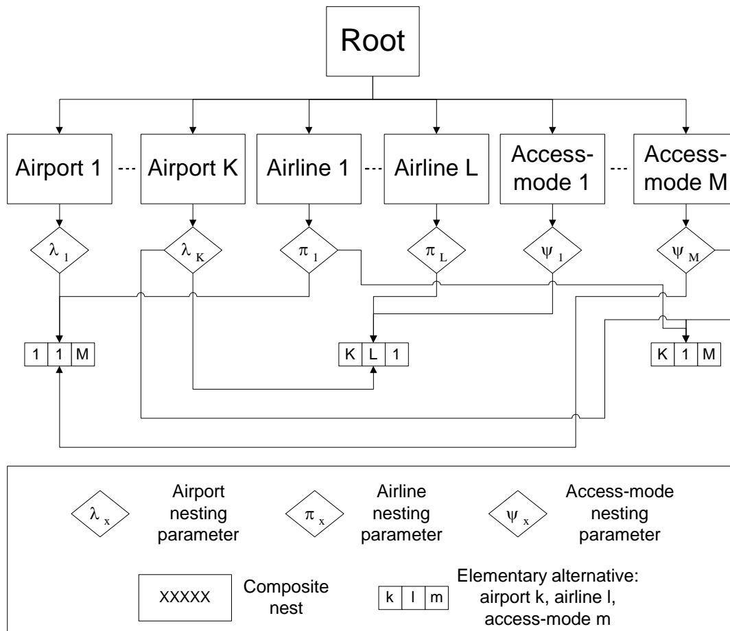
Fig. 2. Structure for cross-nested model
