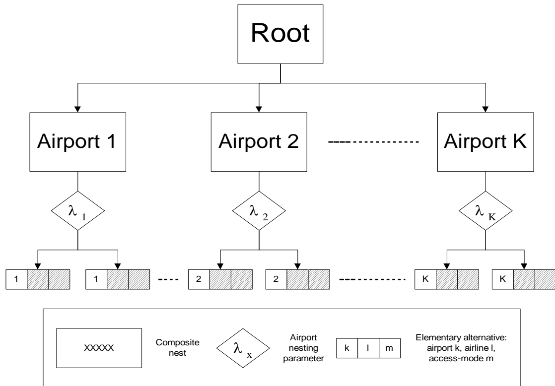
Fig. 1. Structure for models using nesting by airport
