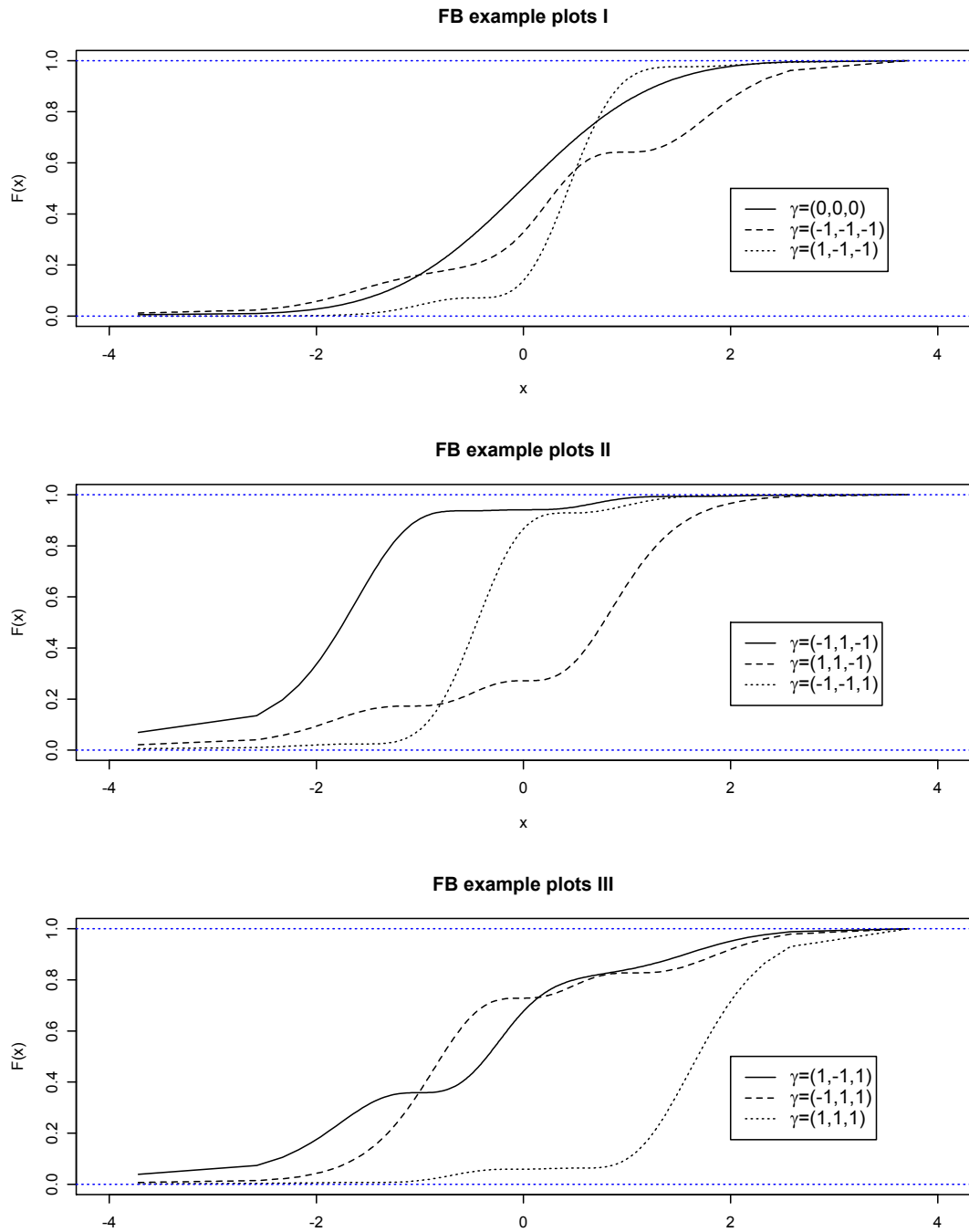
Figure 1: CDF plots for various FB distributions
