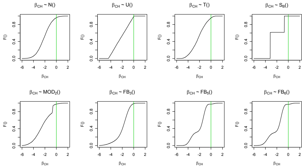
Figure 13: CDF plots for \beta_{CH} in models estimated on Swiss route choice data
