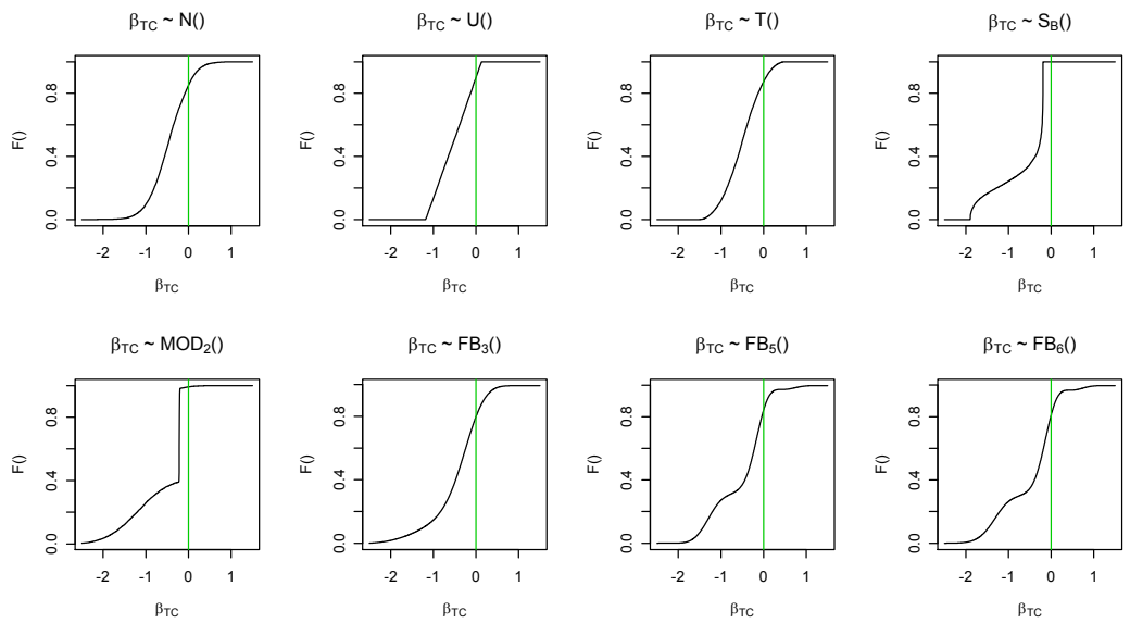
Figure 11: CDF plots for \beta_{TC} in models estimated on Swiss route choice data
