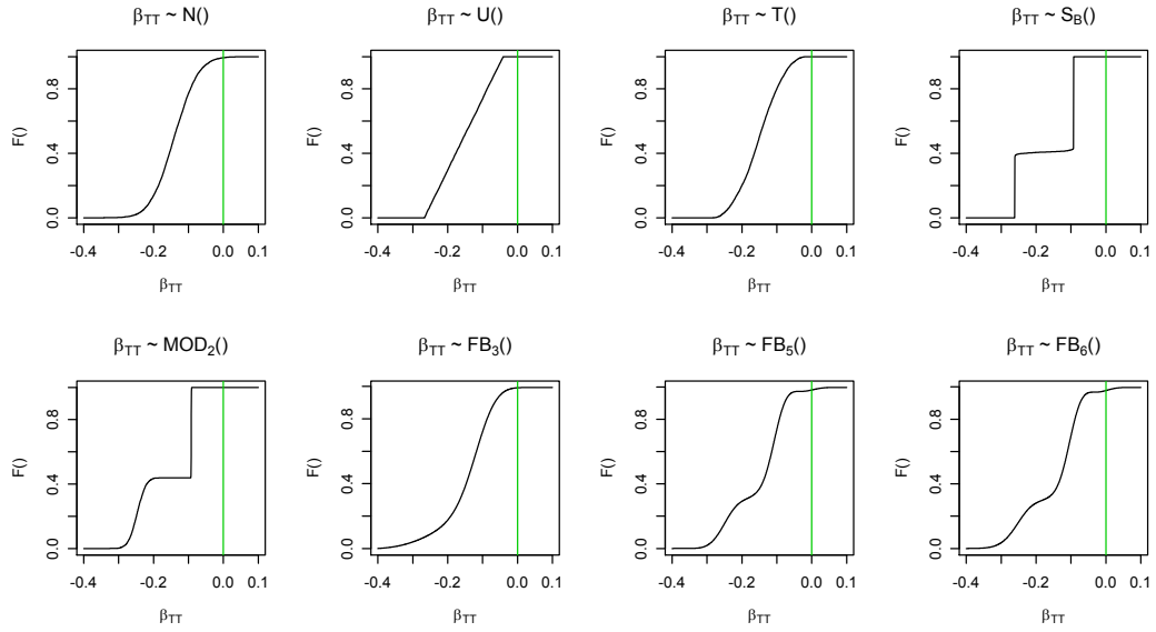
Figure 10: CDF plots for \beta_{TT} in models estimated on Swiss route choice data
